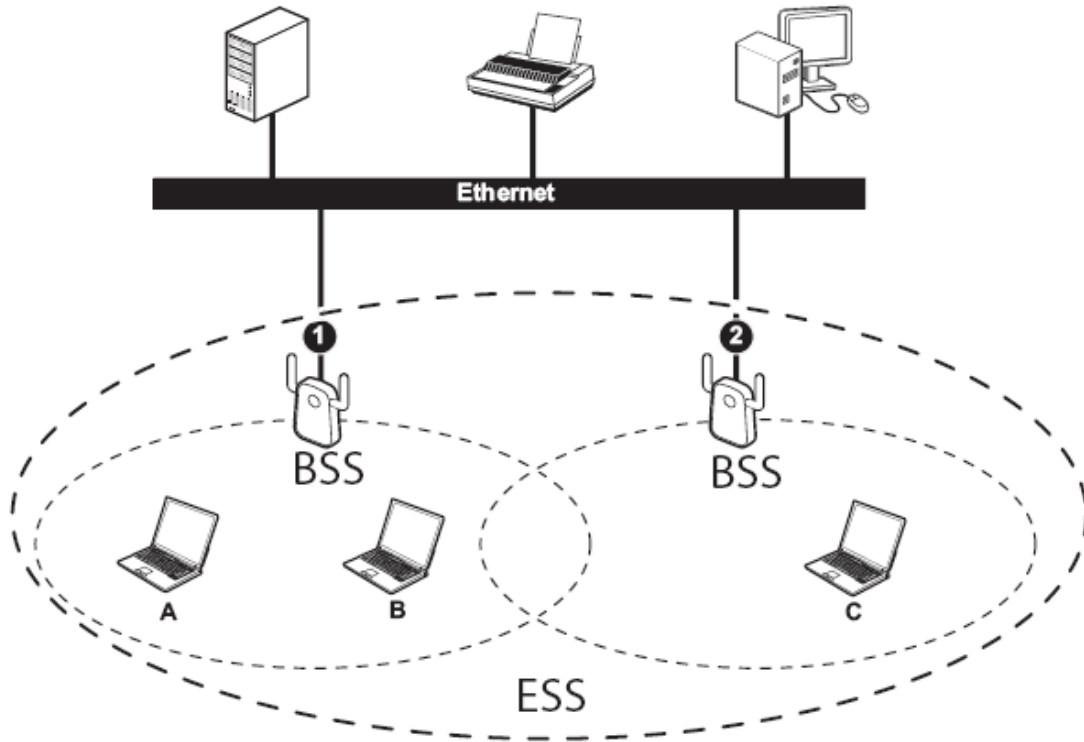
Infrastructure (ESS) network diagram
